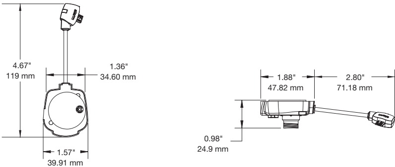
Series 1050 Micro USB Handheld Sensor (DQH200-W):
