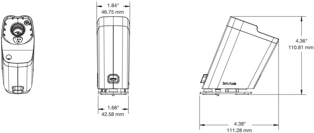
Series 1050 Angled Stand (DQD101-W):
