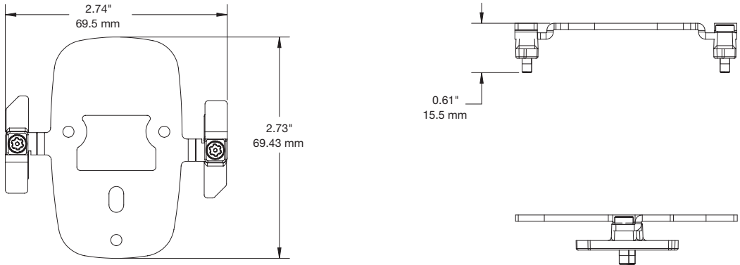
Series 1050 Slot Mount Kit (DQD400):
