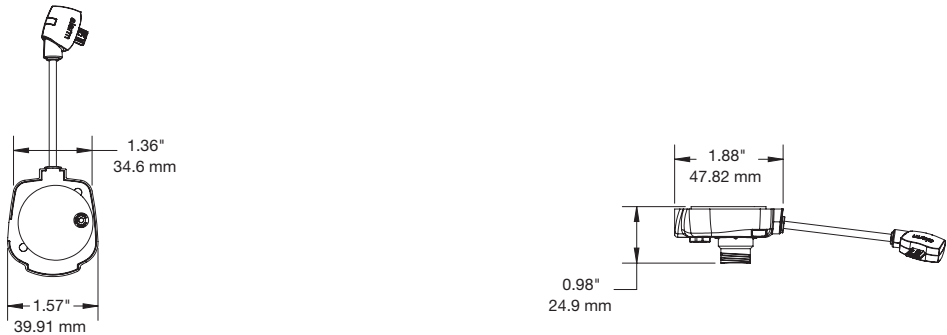
Series 1050 Tablet Micro USB Sensor (DQT200-W):
