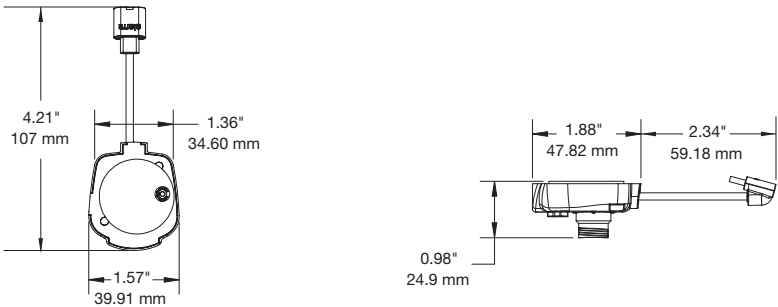
Series 1050 USB Type C Handheld Sensor (DQH202-W):
