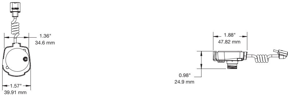
Series 1050 Tablet USB Type C Sensor (DQT202-W):
