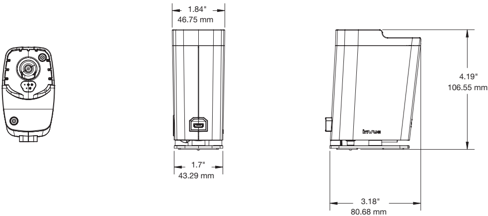
Series 1050 Flat Stand (DQD100-W):
