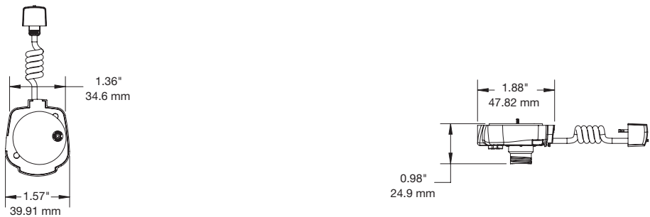
Series 1050 Tablet Apple Lightning Sensor (DQT201-W):
