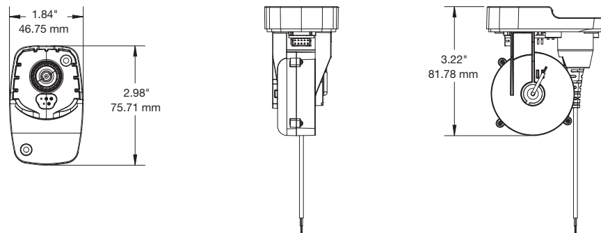
Series 1050 Replacement Recoiler (DQD403-W):
