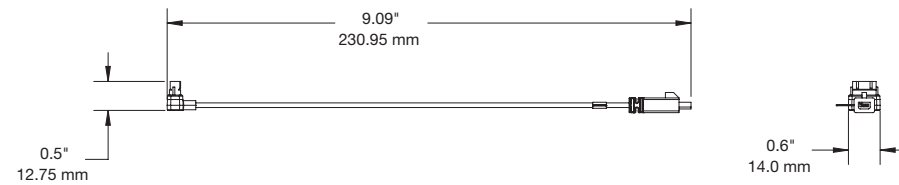
Digital Signage Trigger/Adapter/CCTV Cable (DQD402-W):
