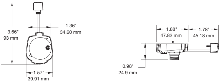
Series 1050 Apple Lightning Handheld Sensor (DQH201-W):
